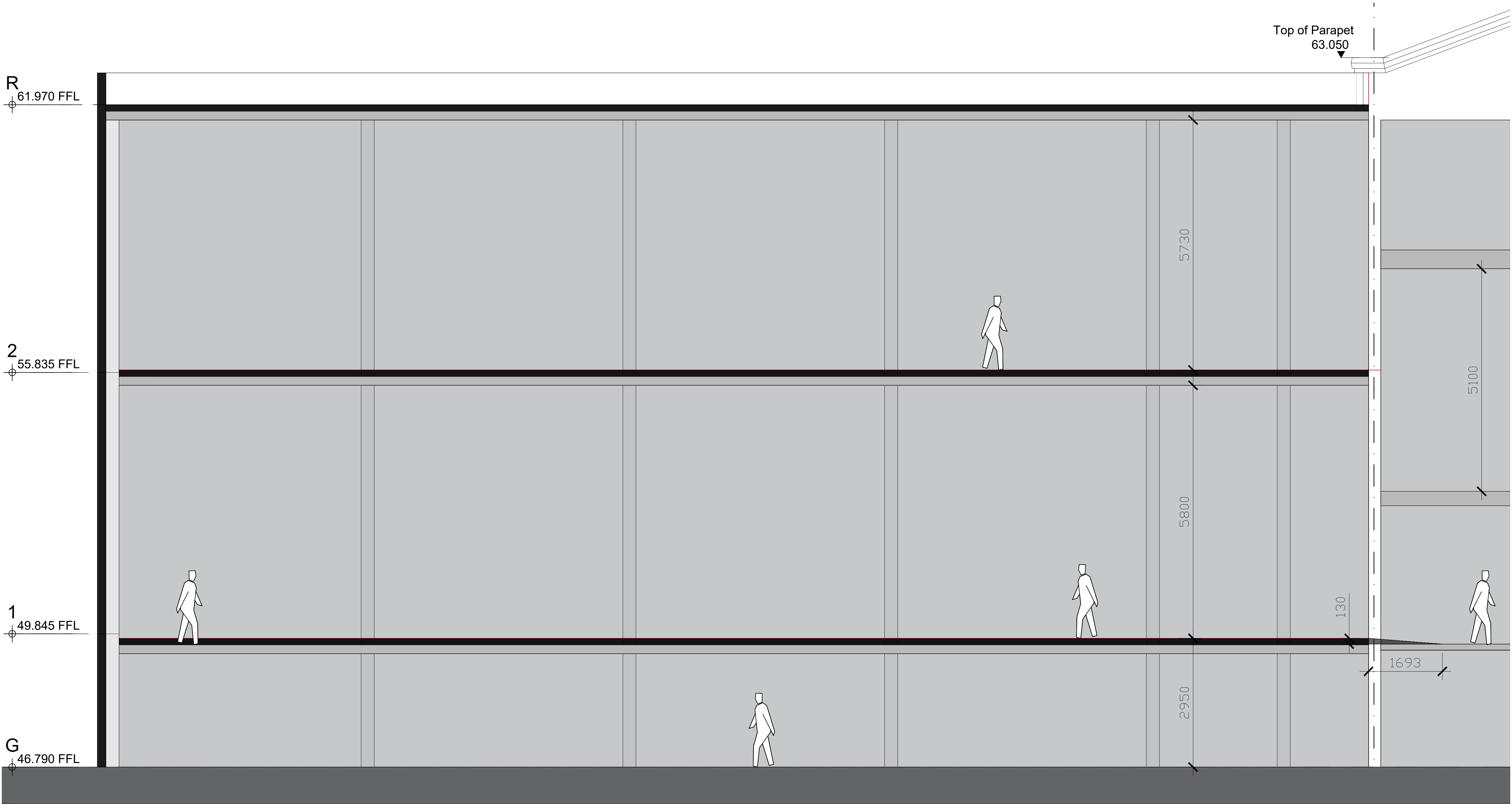
PROPOSED LONG SECTION 1:50
