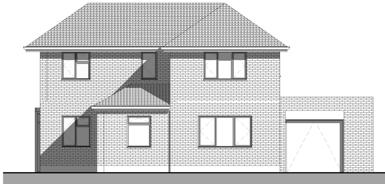
1 Existing Front Elevation 2438-A-101 1 : 100
