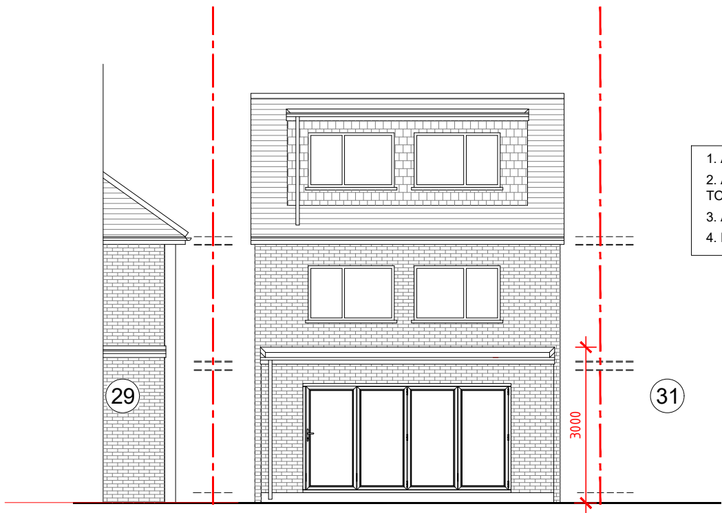
REAR ELEVATION
