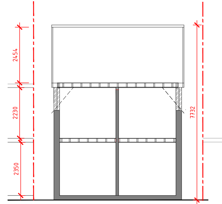
SECTION A - A PROPOSED
