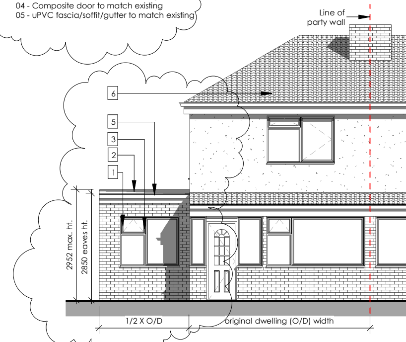
3 Proposed Front Elevation 2403-A-301 1 : 100
