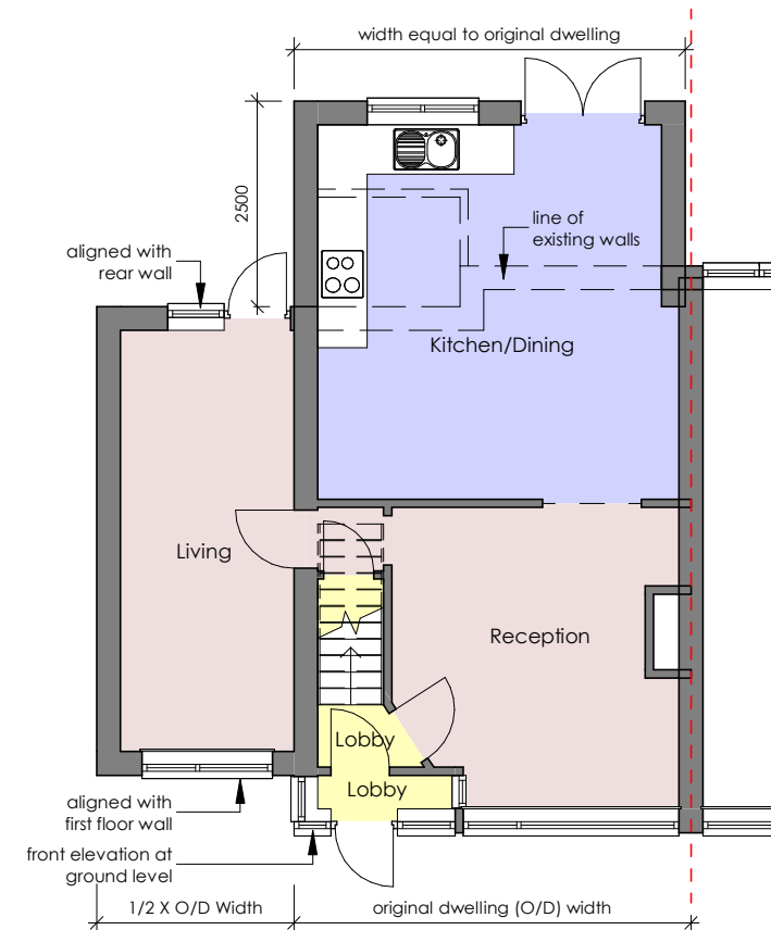
1 Ground Floor (Proposed) 2403-A-301 1 : 100
