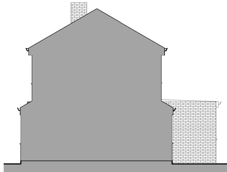
4 Proposed Side Elevation (no. 95) 2403-A-301 1 : 100
