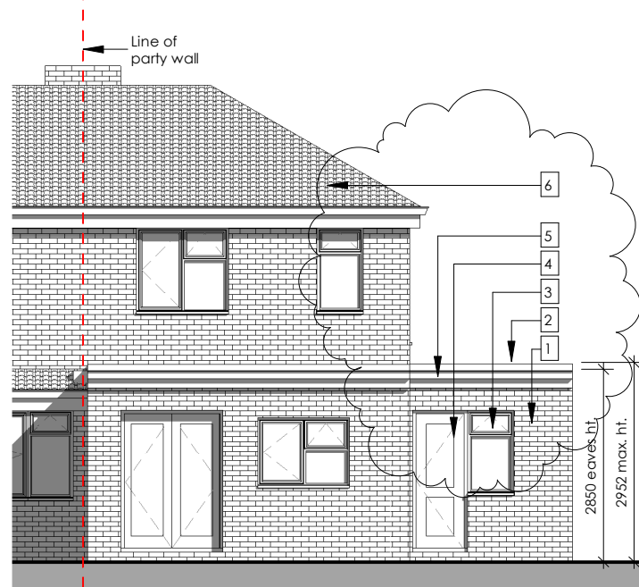
5 Proposed Rear Elevation 2403-A-301 1 : 100
