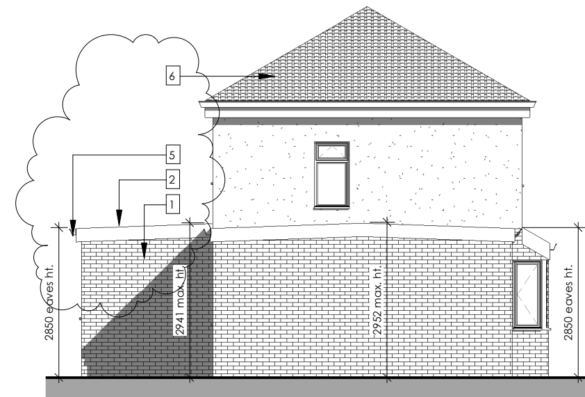
6 Proposed Side Elevation 2403-A-301 1 : 100
