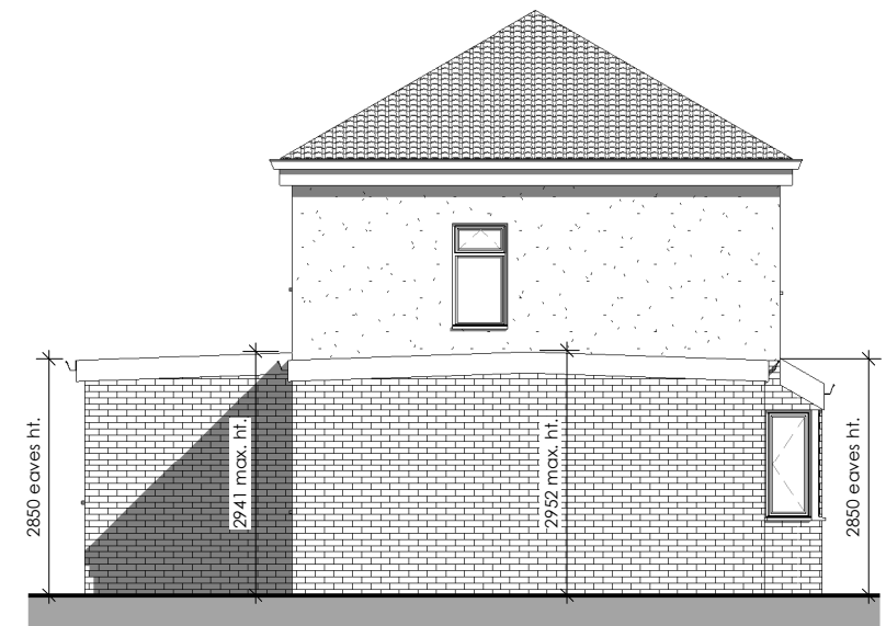
6 Proposed Side Elevation 2403-A-301 1 : 100
