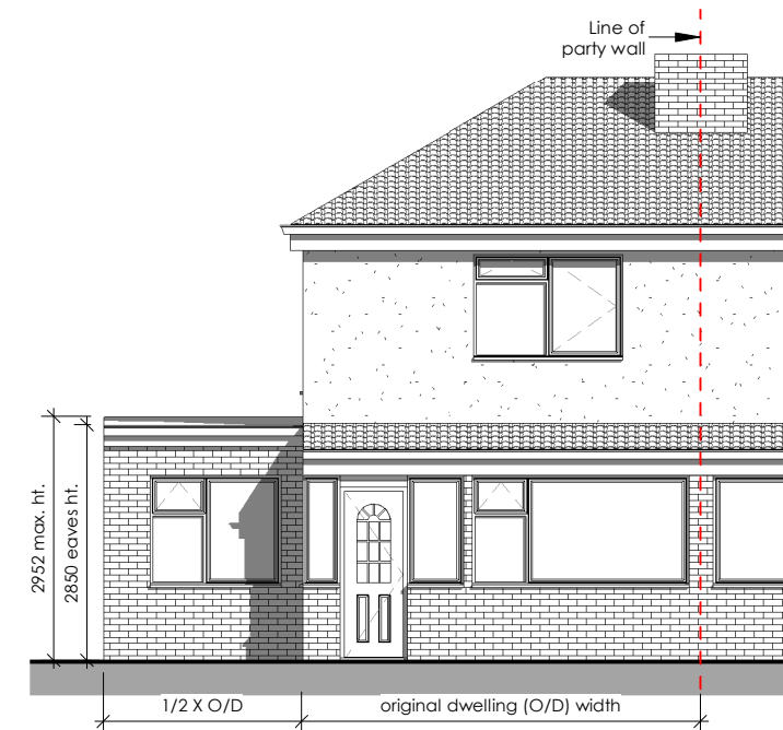
3 Proposed Front Elevation 2403-A-301 1 : 100
