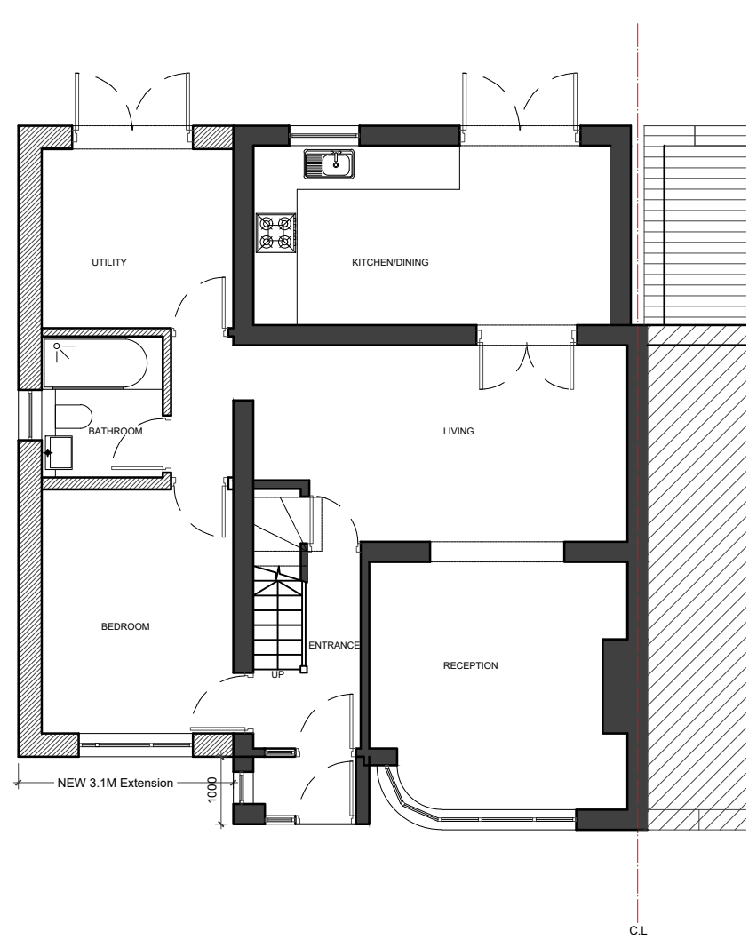
01-GROUND FLOOR PLAN
