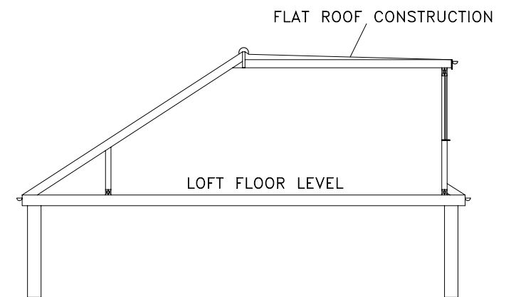
LOFT SECTION
