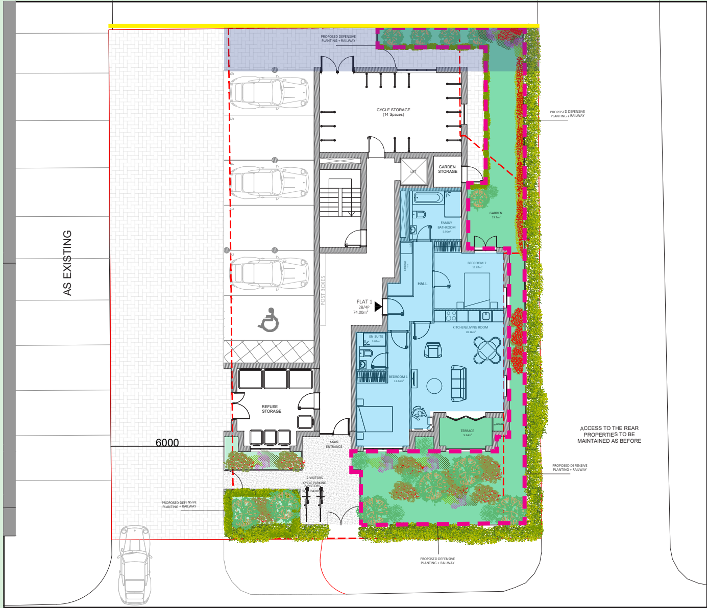
APPLICATION REFERENCE: PROPOSED DESIGN 2024 PROPOSED GROUND FLOOR PLAN
