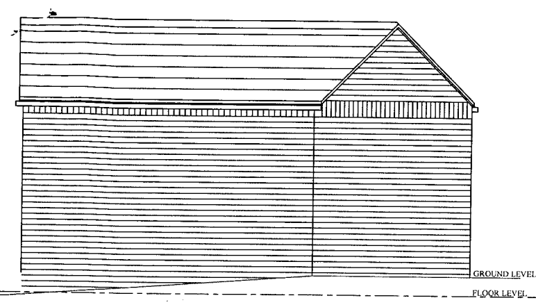
PROPOSED OTHER SIDE ELEVATION 1:100
