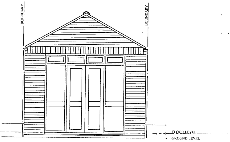
PROPOSED GARDEN ELEVATION 1:100
