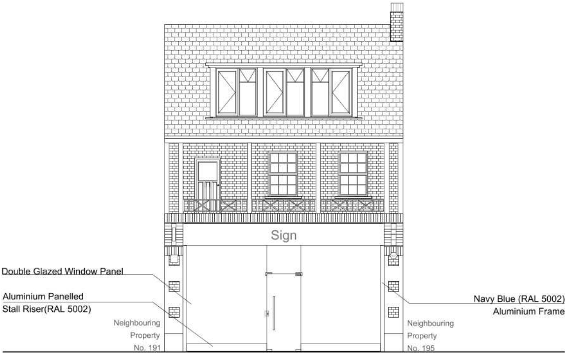
EXISTING / PROPOSED FRONT ELEVATION
