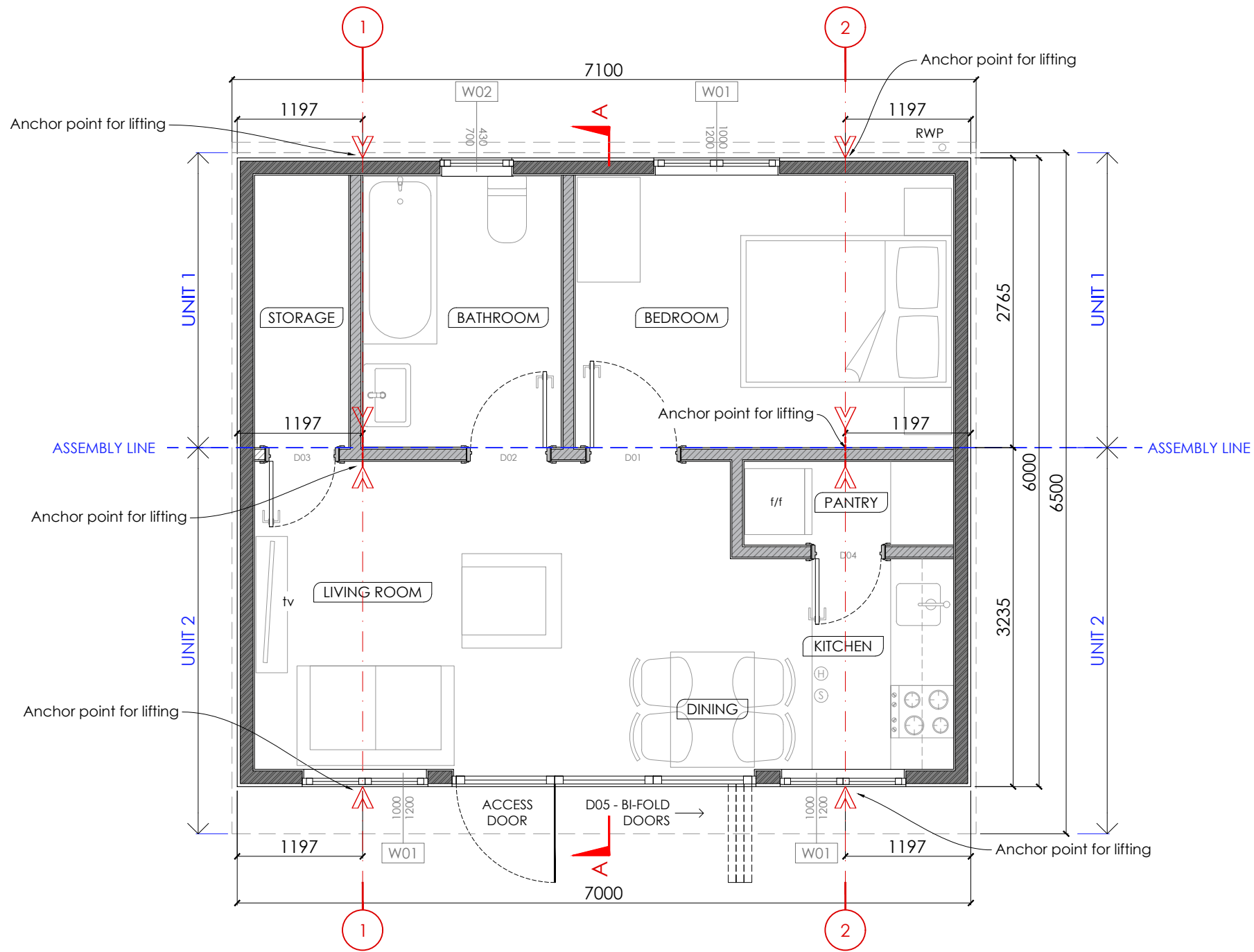
LAYOUT PLAN
