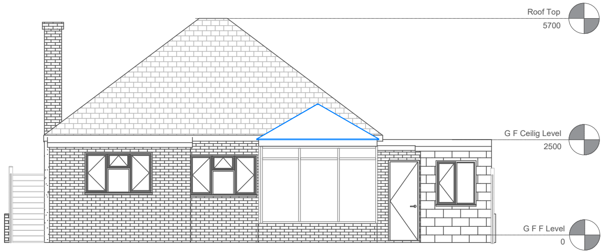
BACK ELEVATION - EXISTING
