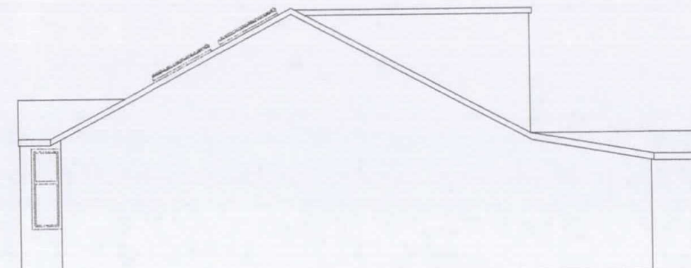
EXISTING RIGHT SIDE ELEVATION
