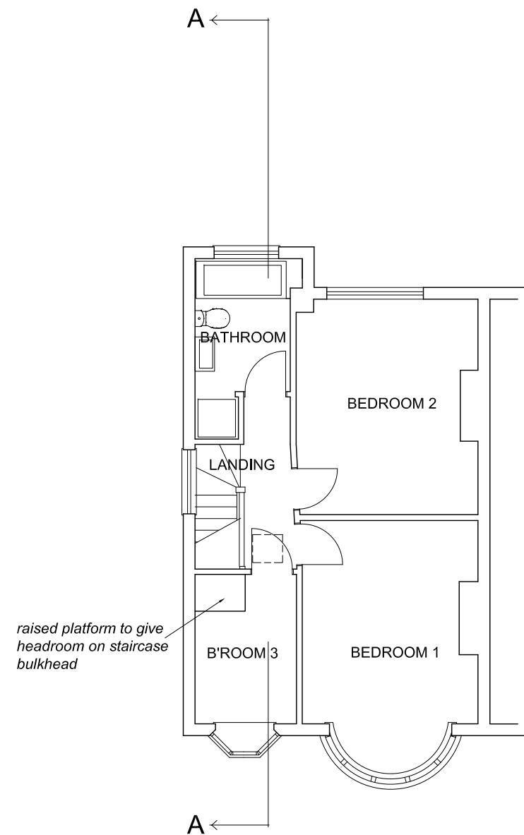
FIRST FLOOR PLAN - EXISTING
