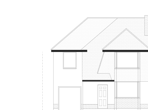
PROPOSED FRONT ELEVATION
