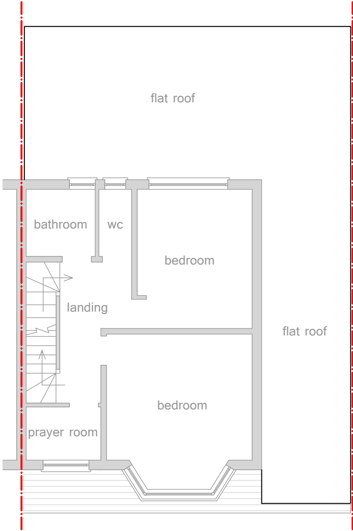
Existing First Floor
