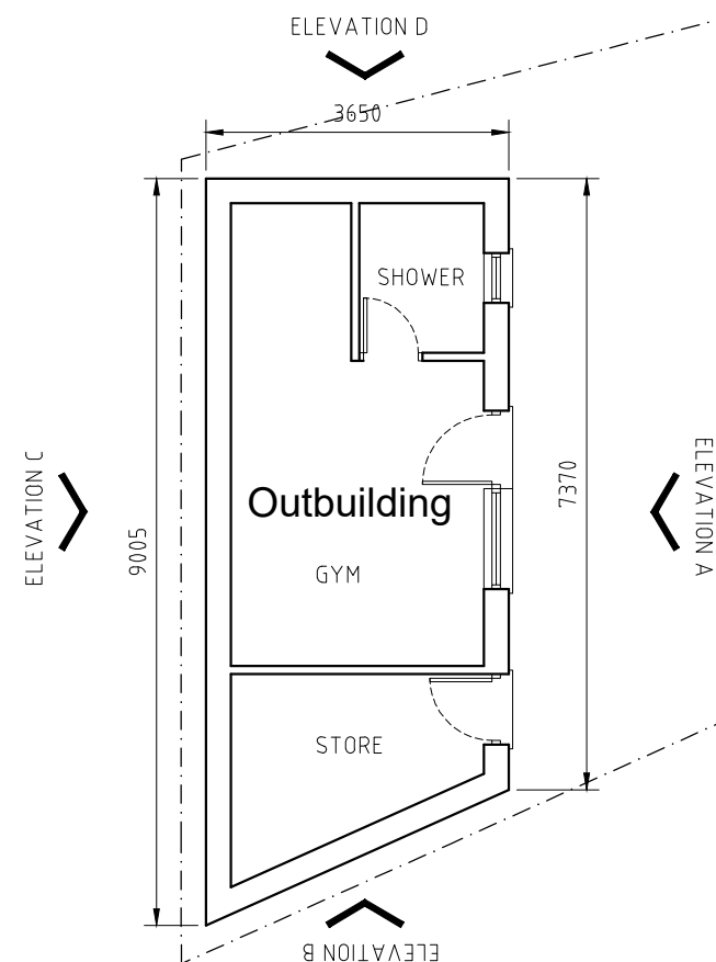
PROPOSED OUTBUILDING PLAN
