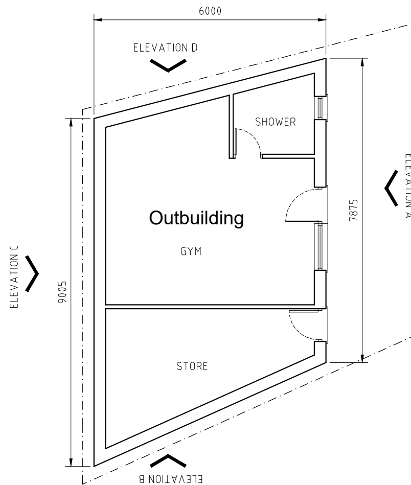
PROPOSED OUTBUILDING PLAN
