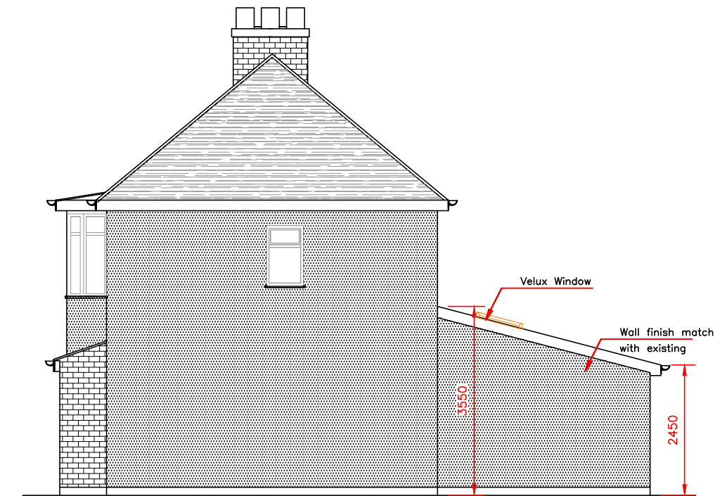
PROPOSED SIDE ELEVATION From No-80 SCALE:-1:100
