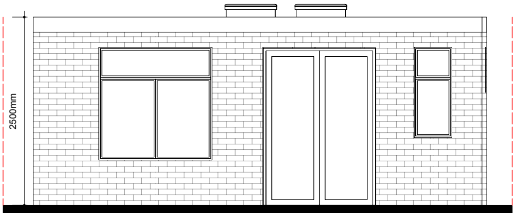
1 Front Elevation 1:50
