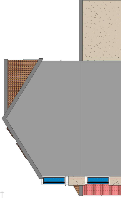
4 1 : 100 Existing Flank Wall_Elevation
