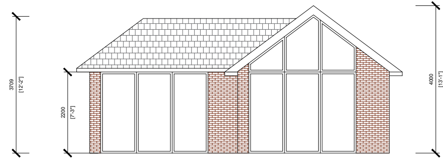
PROPOSED FRONT ELEVATION 1:100
