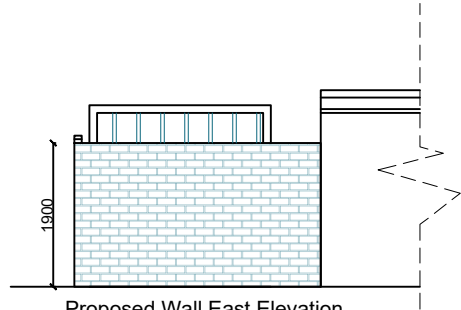
Proposed Wall East Elevation
