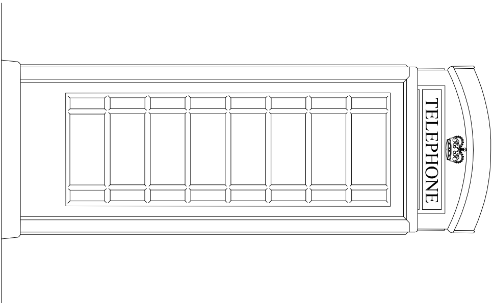
Proposed Side Elevation 1 @ 1 : 20
