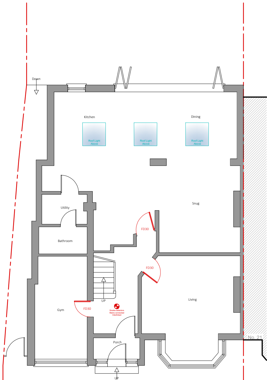
1 Proposed Ground Floor Plan
