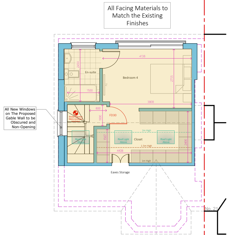
3 Proposed Loft Floor Plan
