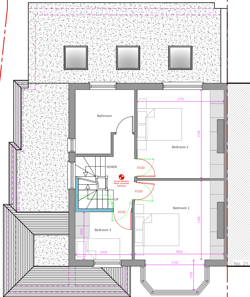
2 Proposed First Floor Plan
