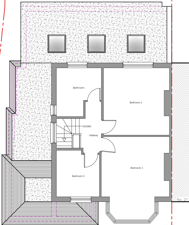
2 Existing First Floor Plan
