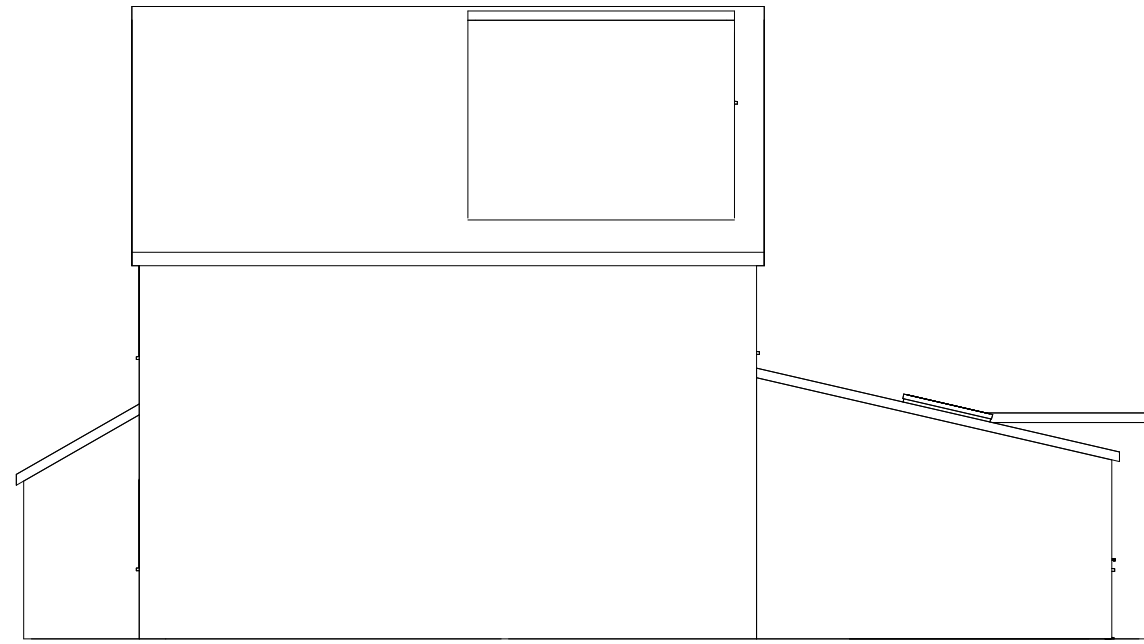
8 East Elevation Proposed 1 : 100
