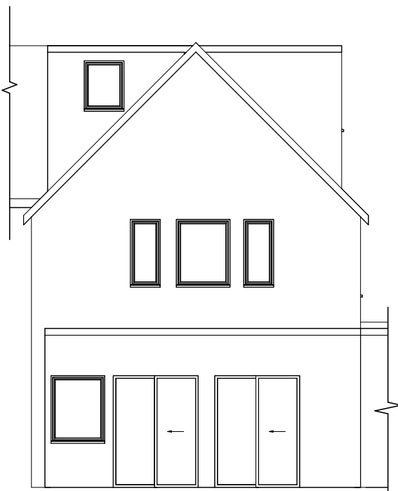
5 Rear Elevation Existing 1 : 100
