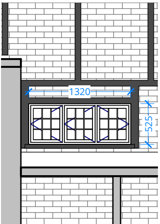
EXISTING OPENING TYPE EO 48
