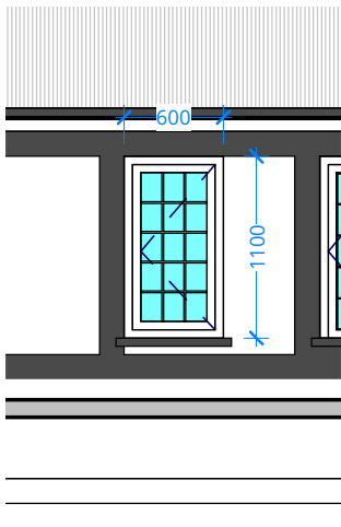
OPENING TYPE EO 58
