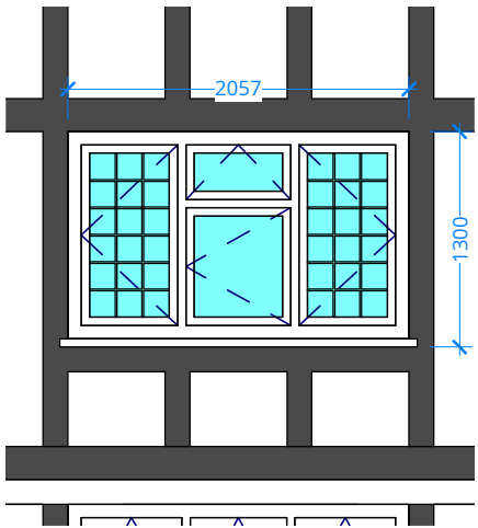
OPENING TYPE EO 60
