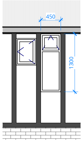
PROPOSED - TO MATCH EXISTING
