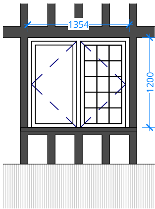
EXISTING OPENING TYPE EO 38
