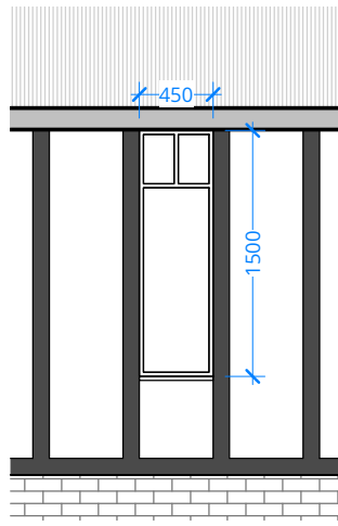
OPENING TYPE EO 36
