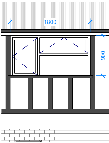
OPENING TYPE EO 35
