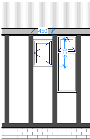
EXISTING OPENING TYPE EO 39
