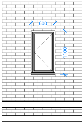
OPENING TYPE EO 33
