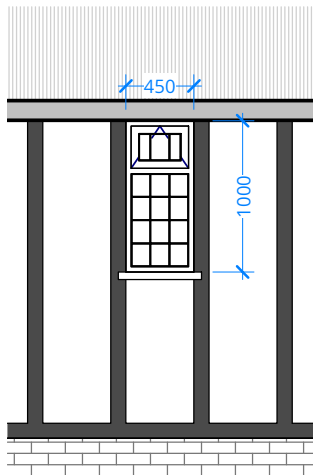
OPENING TYPE EO 37
