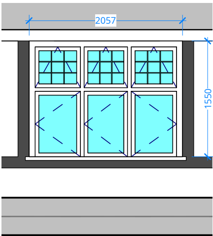
OPENING TYPE EO 31
