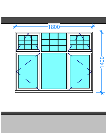
OPENING TYPE EO 28
