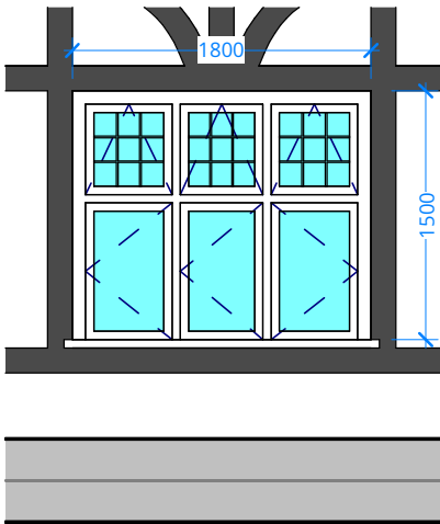
OPENING TYPE EO 30
