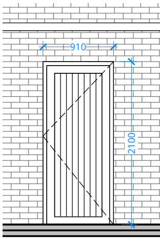
OPENING TYPE EO 26
