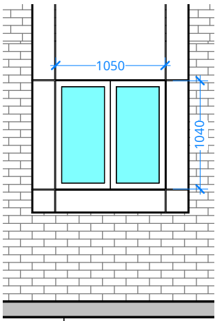
OPENING TYPE EO 27
