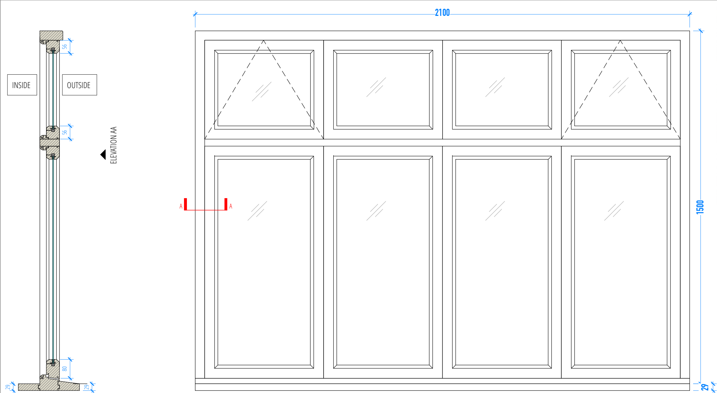
01 TUDOR SUITE WINDOW SECTION A-A 1:10 @ A3
