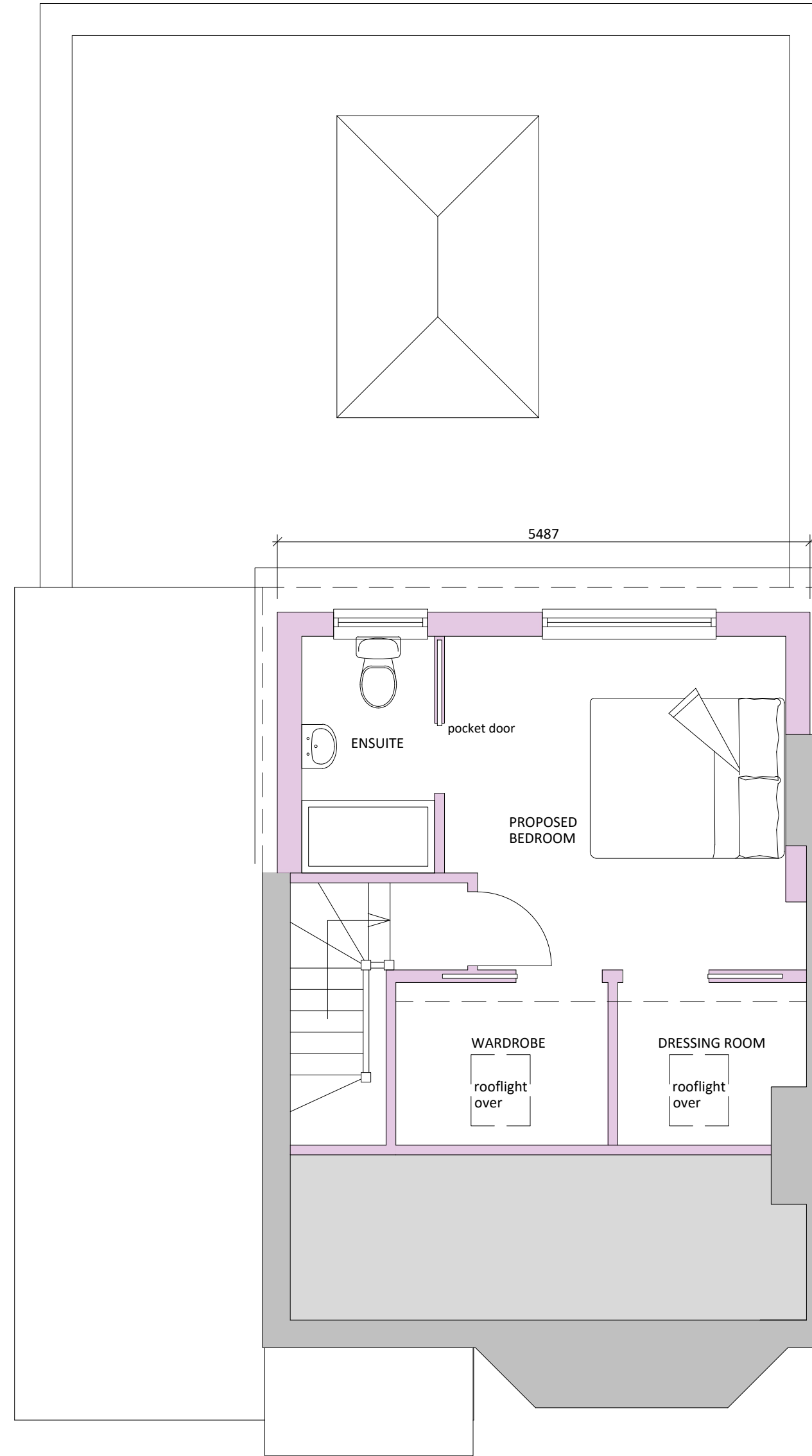
SECOND FLOOR PLAN - PROPOSED
