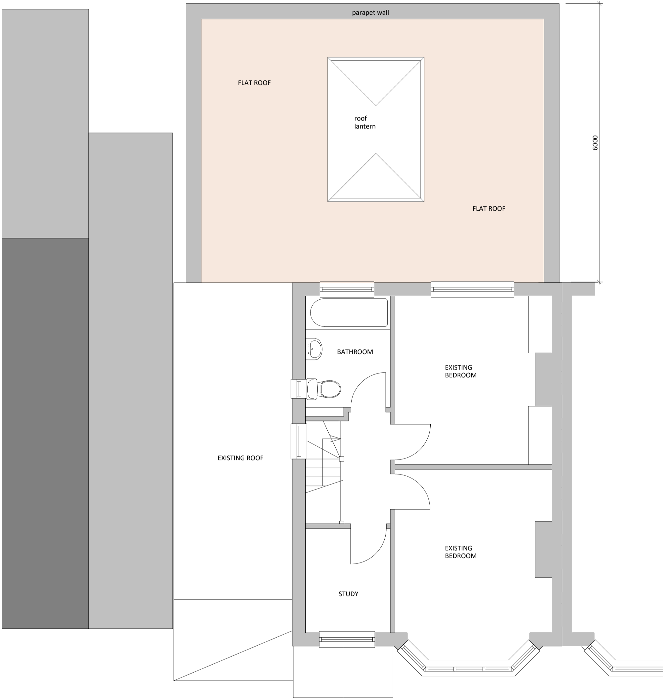
FIRST FLOOR PLAN - UNCHANGED
