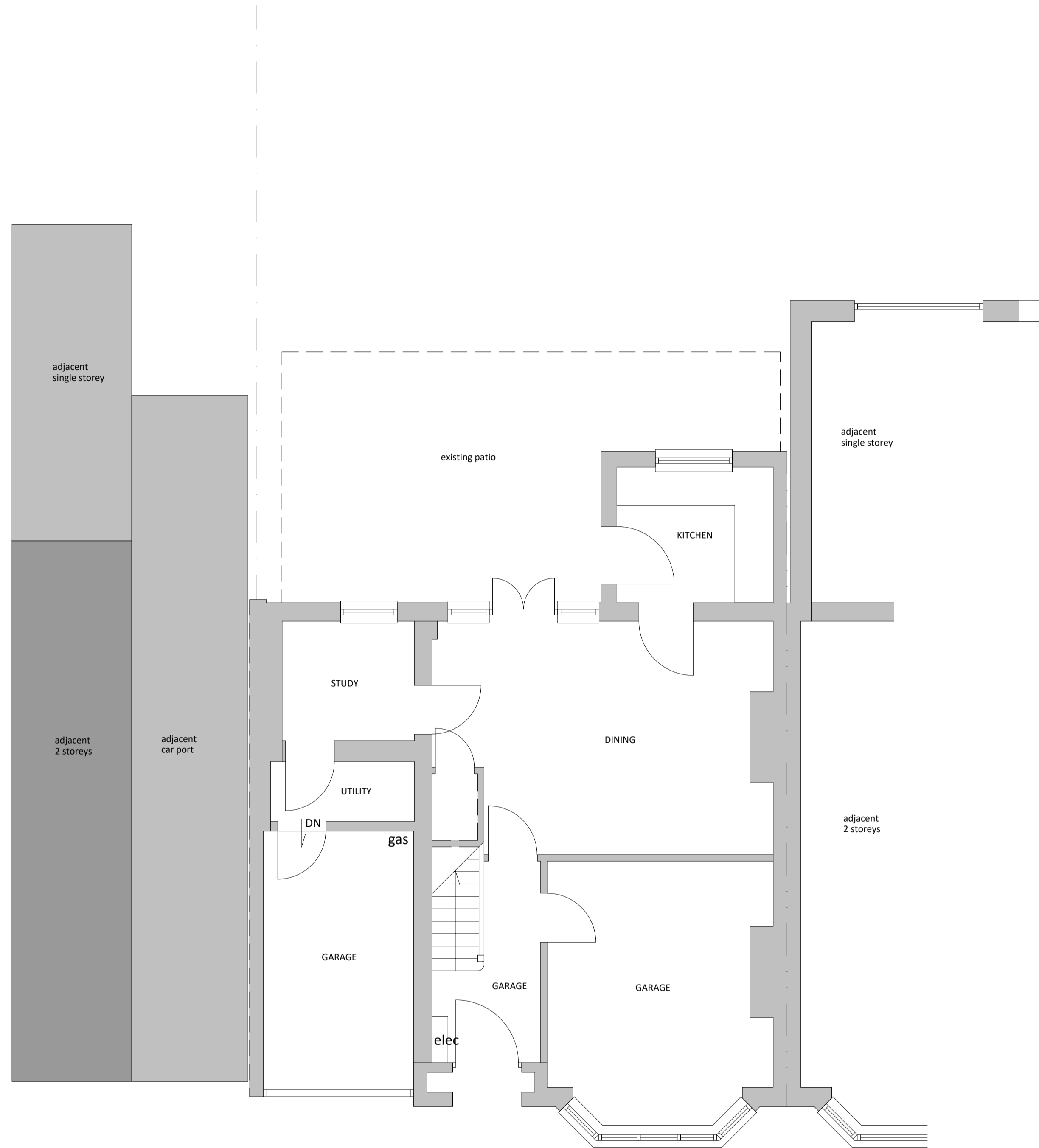
GROUND FLOOR PLAN - UNCHANGED
