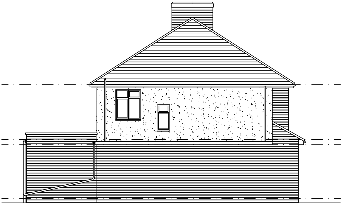
PRE-EXISTING SIDE ELEVATION 1
