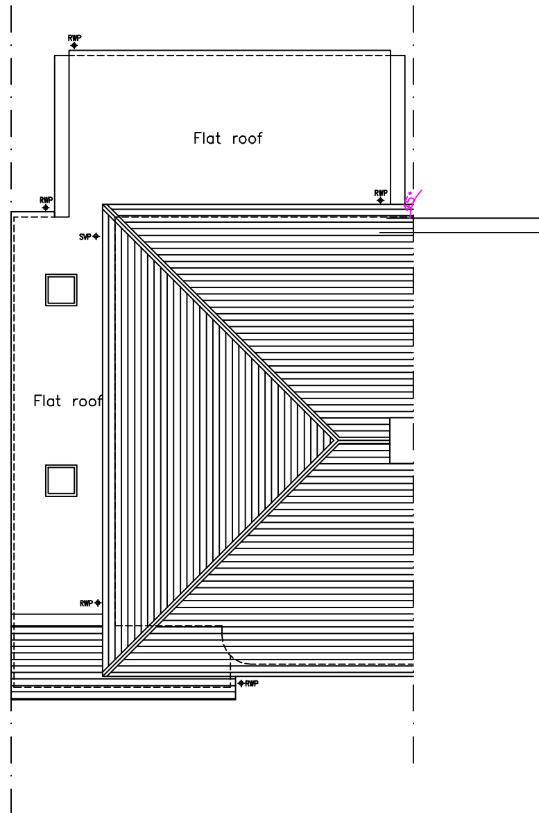
PRE-EXISTING ROOF PLAN
