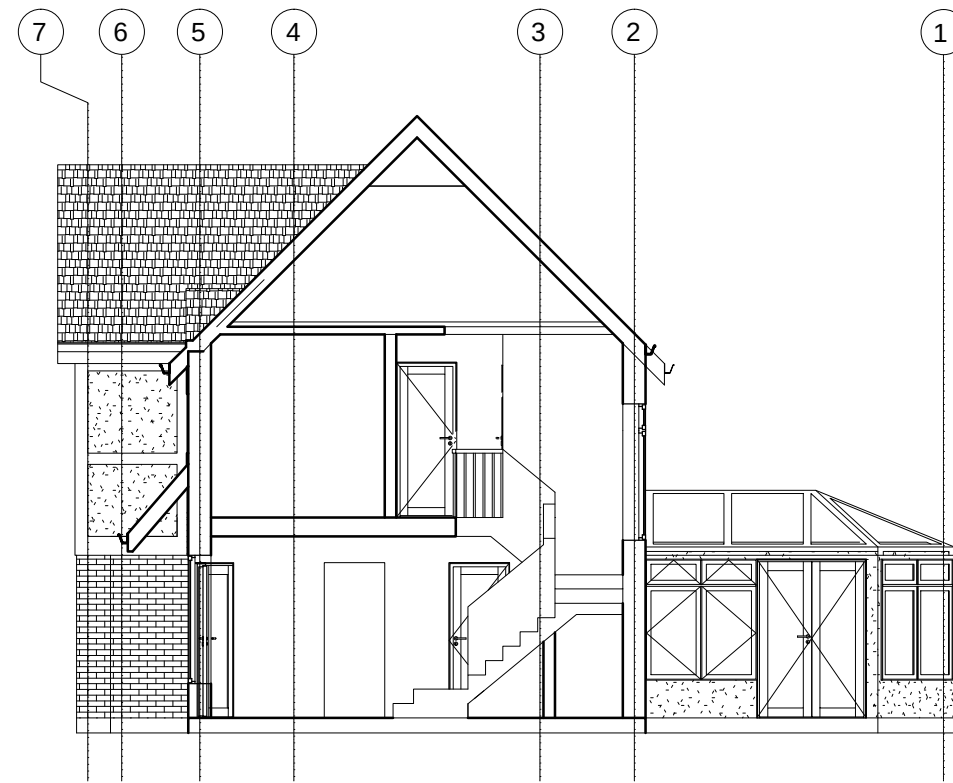
EXISTING SECTION
