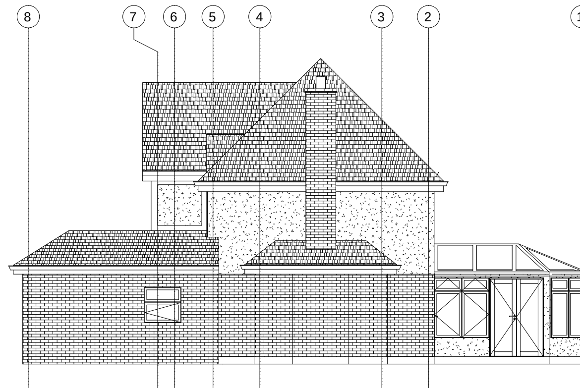
EXISTING RIGHT LEFT ELEVATION
