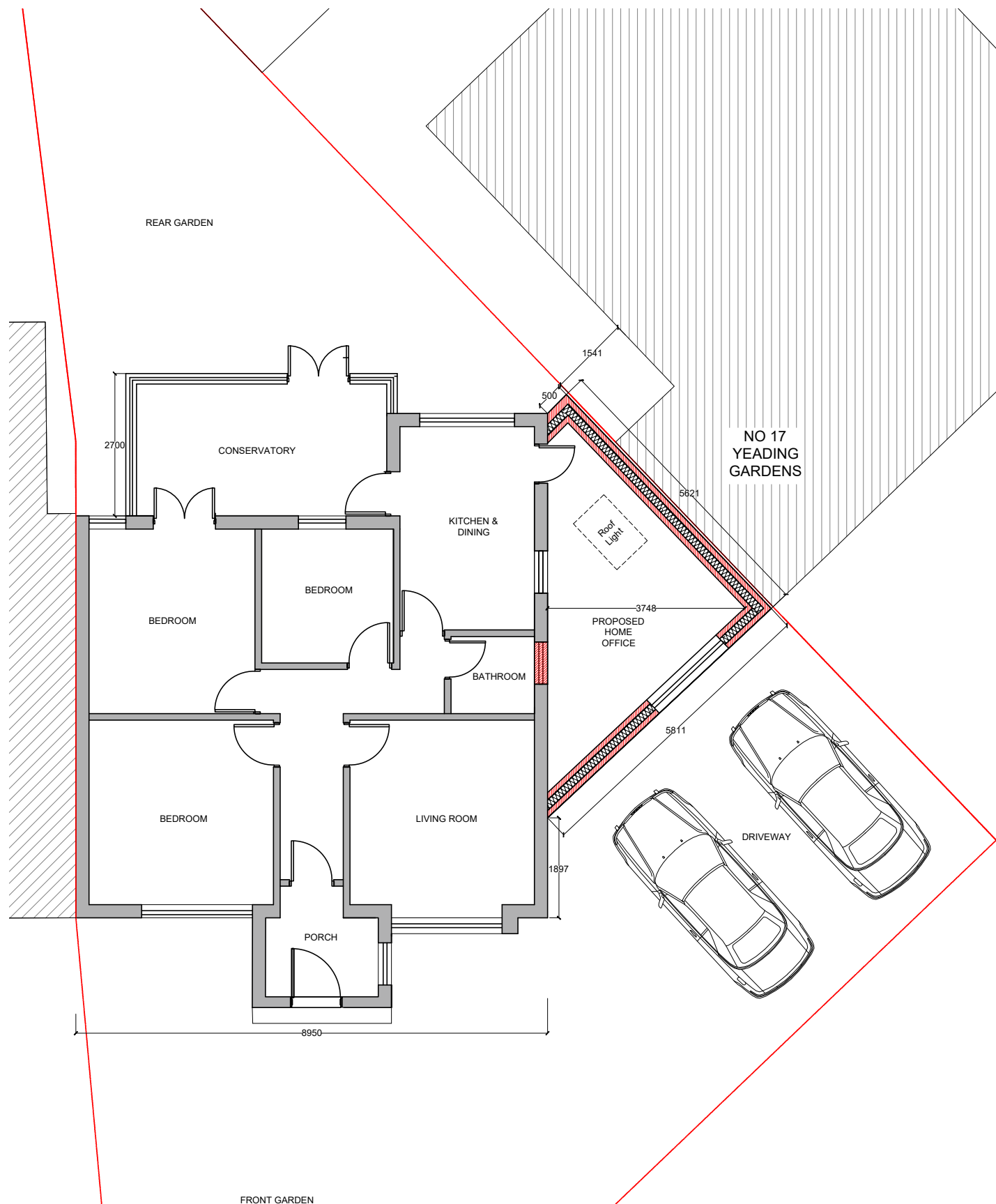
A Proposed Ground Floor Scale: 1:100
