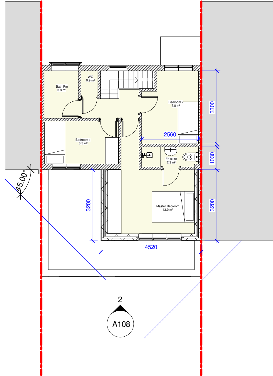
2 PROPOSED FIRST FLOOR PLAN 1 : 100
