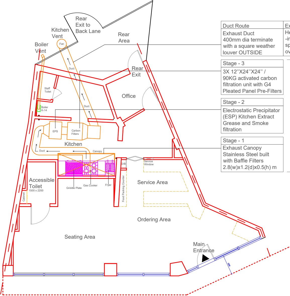
GROUND FLOOR EXTRACTOR VENTILATION PROPOSAL PLAN
