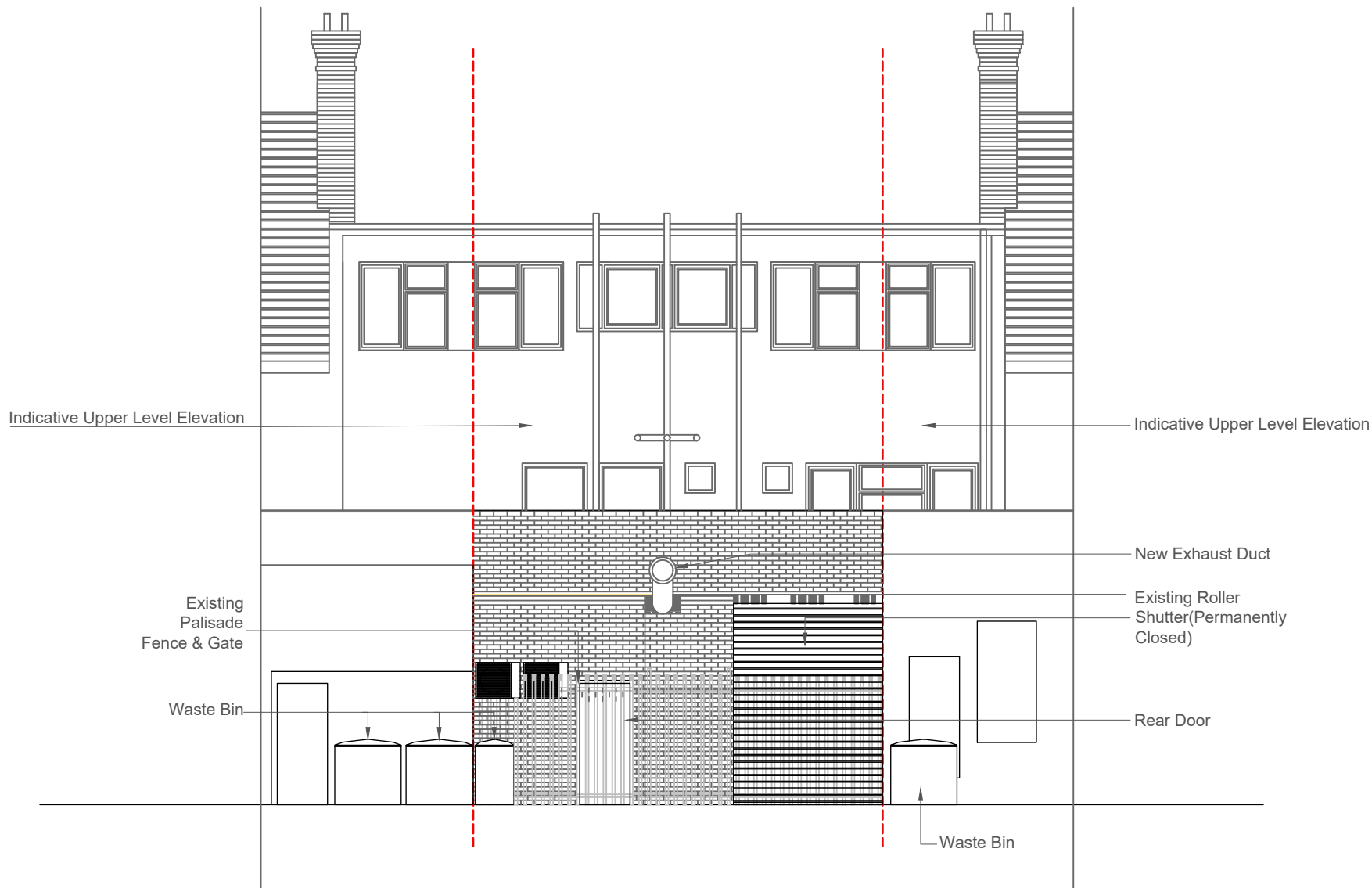
PROPOSED REAR (SOUTH) ELEVATION
