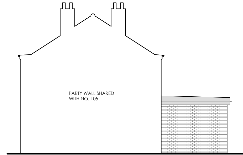
PROPOSED OPPOSITE SIDE ELEVATION
