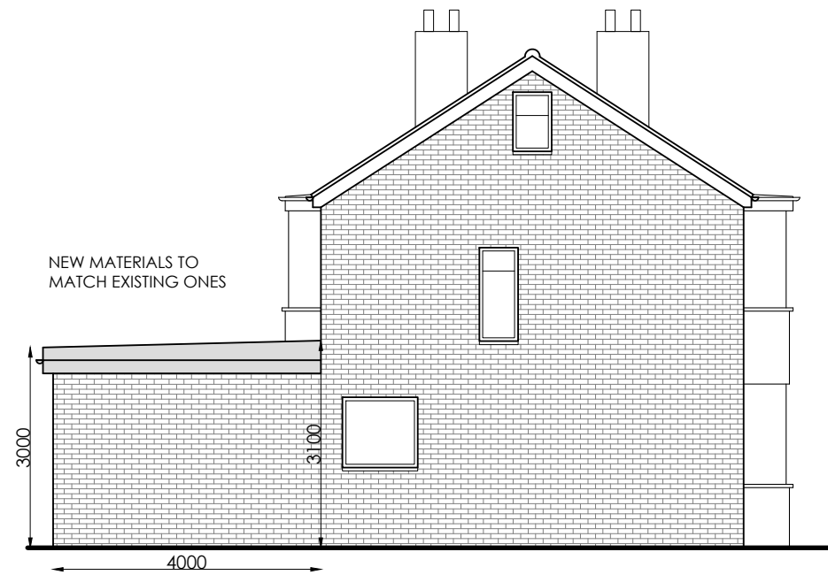
PROPOSED FLANK ELEVATION
