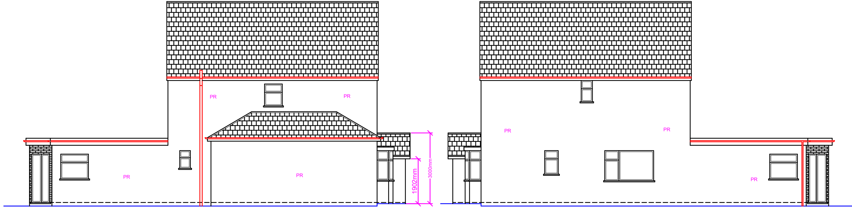
Proposed Side Elevation (LHS)
