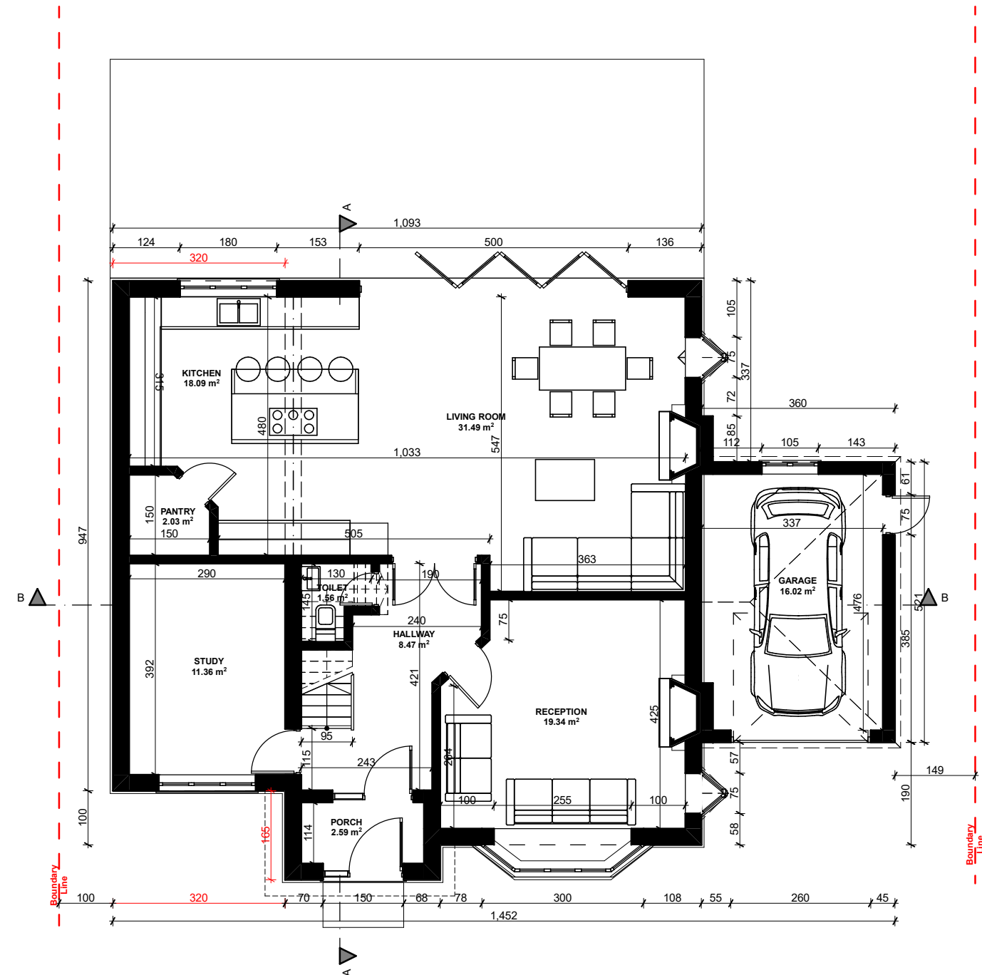
GROUND FLOOR
