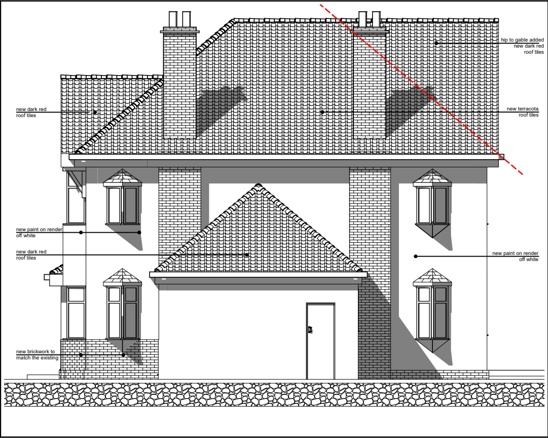
SIDE ELEVATION
