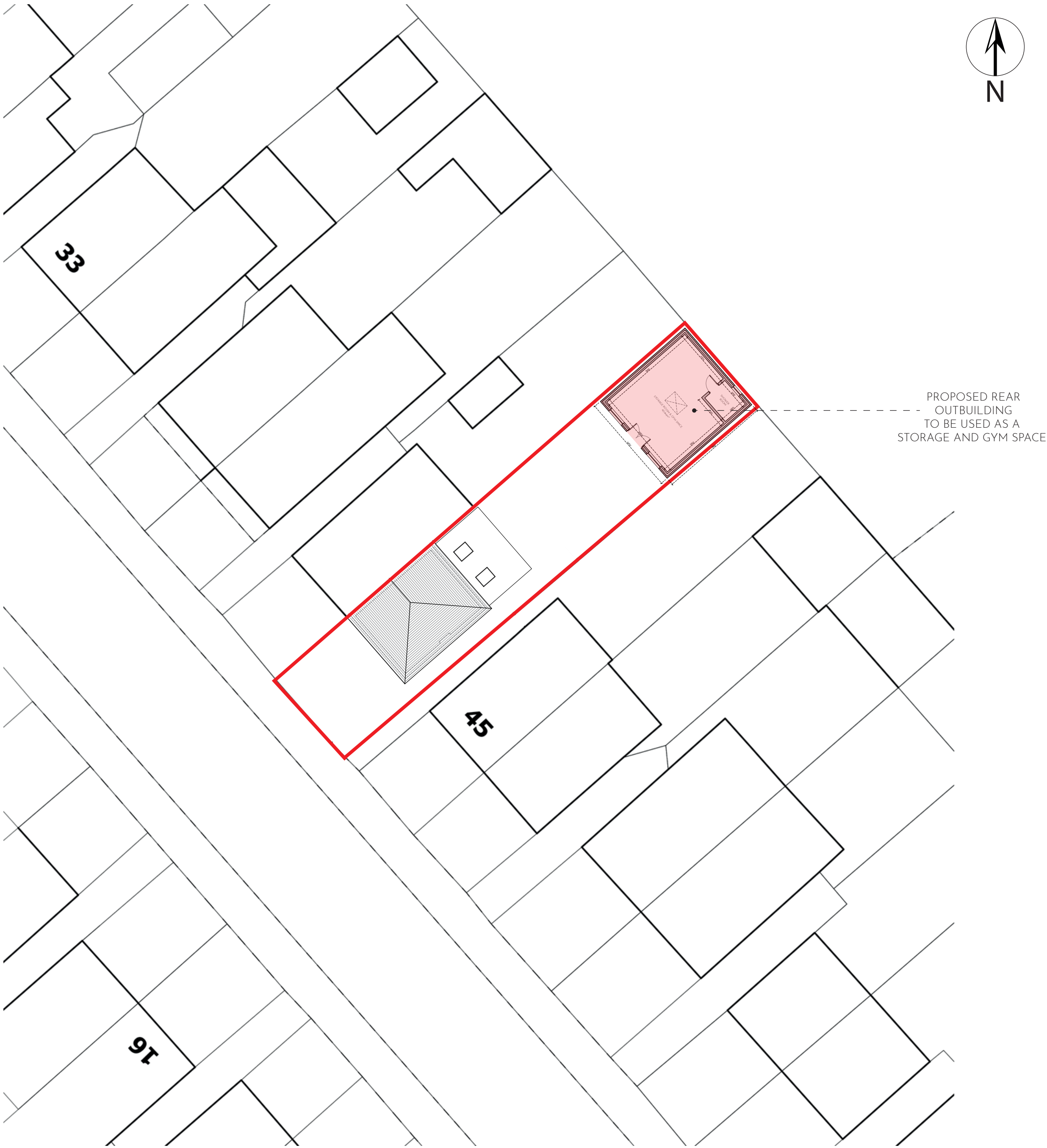
PROPOSED SITE BLOCK PLAN SCALE 1:200
