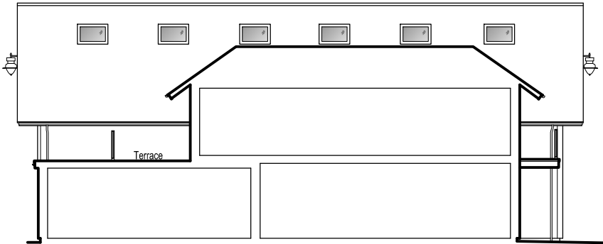
PROPOSED ELEVATION-SECTION 5
