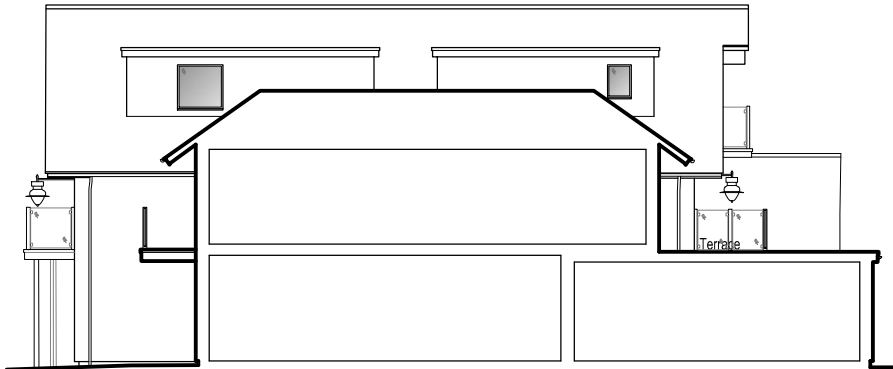
PROPOSED ELEVATION-SECTION 6
