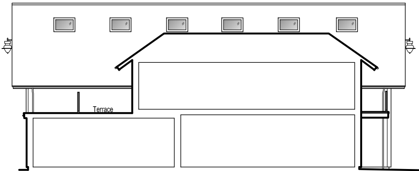
PROPOSED ELEVATION-SECTION 5
